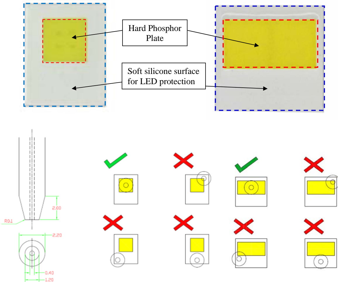
Figure 3: Recommended LED Pick & Place Nozzle Size And Pick Up Position For NagaJo 2025 & NagaJo 2725
