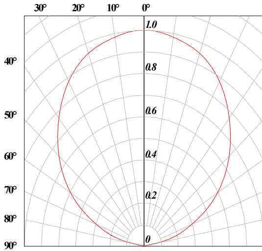
Radiation Pattern
