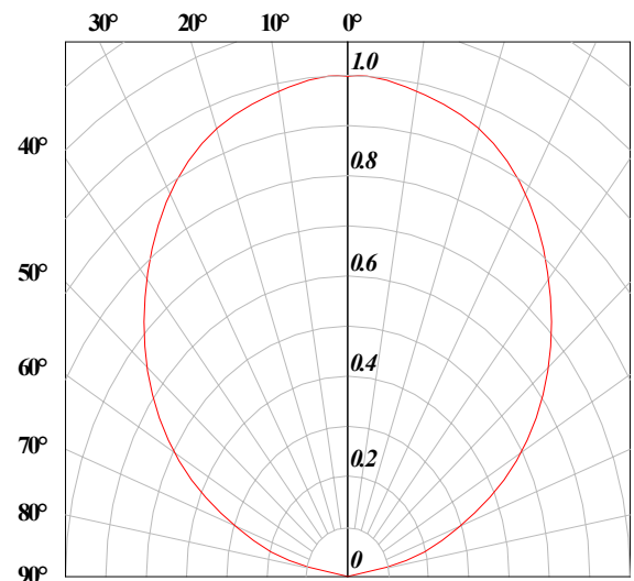
Radiation Pattern
