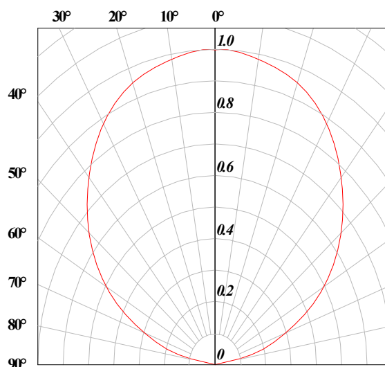
Radiation Pattern
