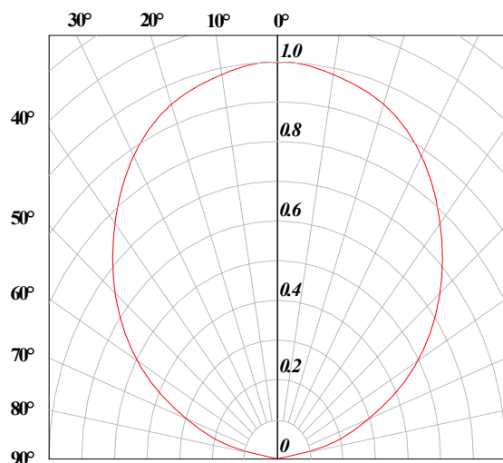
Radiation Pattern
