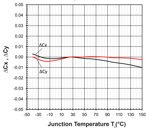
Chromaticity Coordinate Shift Vs Junction Temperature
