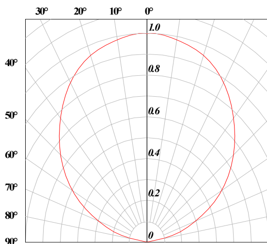
Radiation Pattern
