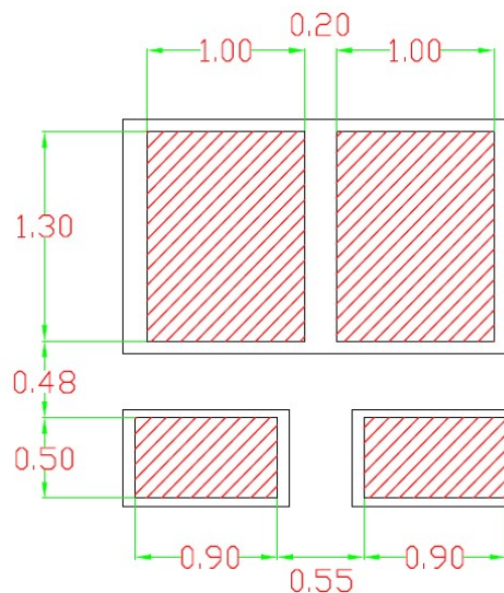
Recommended Solder Stencil Design
