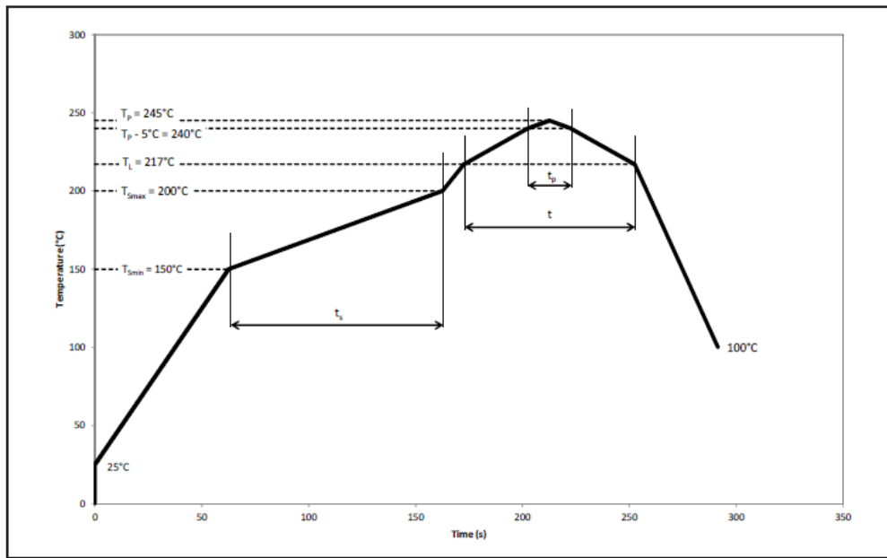
Figure 1: Recommended Pb-free Soldering Profile
