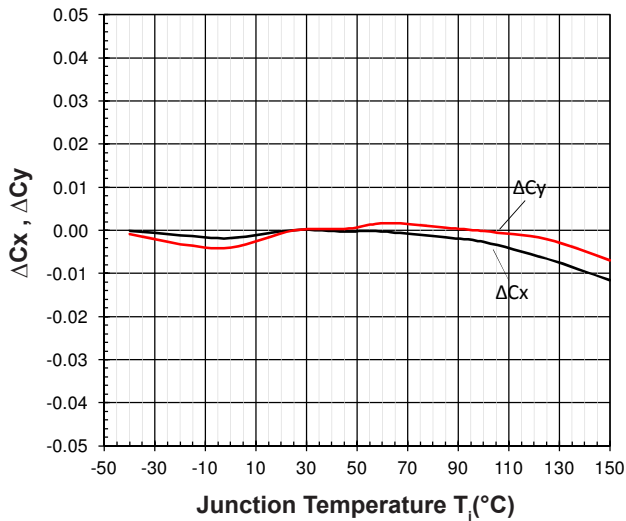
Chromaticity Coordinate Shift Vs Junction Temperature
