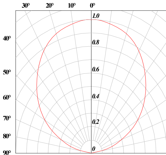
Radiation Pattern
