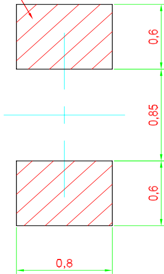
Recommended Solder-pad
